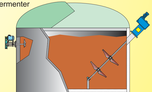
Hold-up Tank
