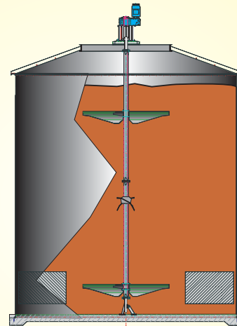
Buffer Tank
